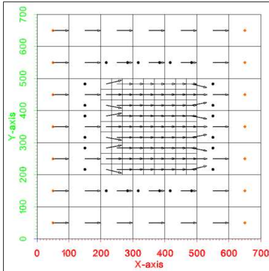
Figure 6 Velocity vectors
