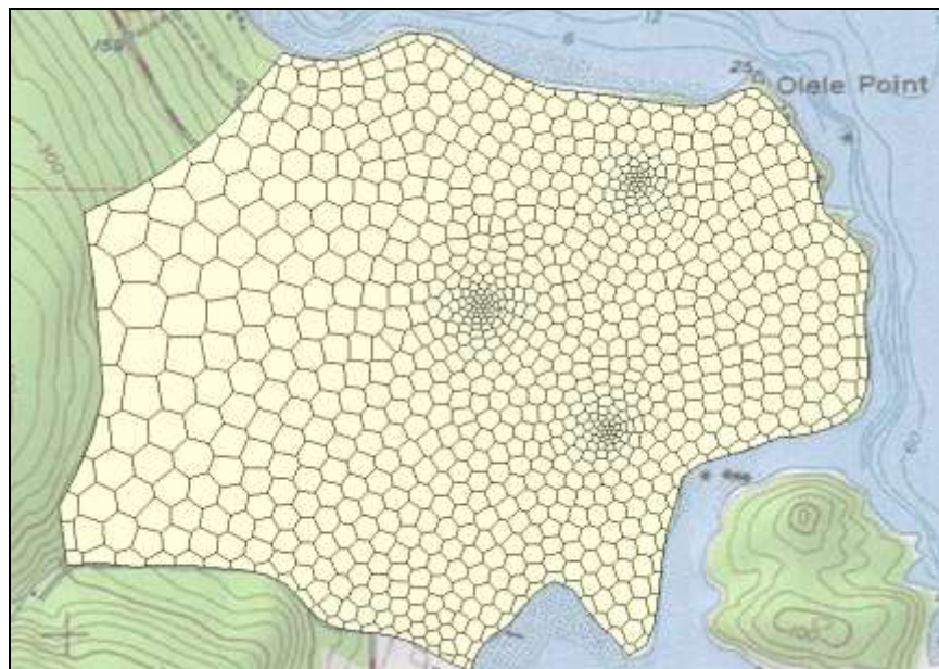
Figure 12 2D Voronoi UGrid
