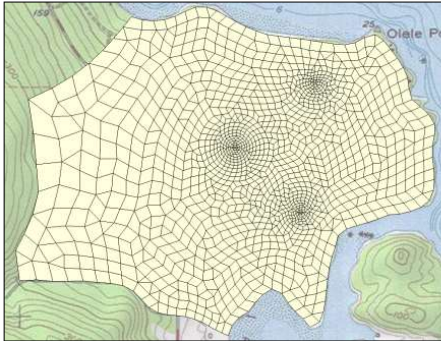
Figure 16 UGrid comprising triangle and quadrilateral cells
