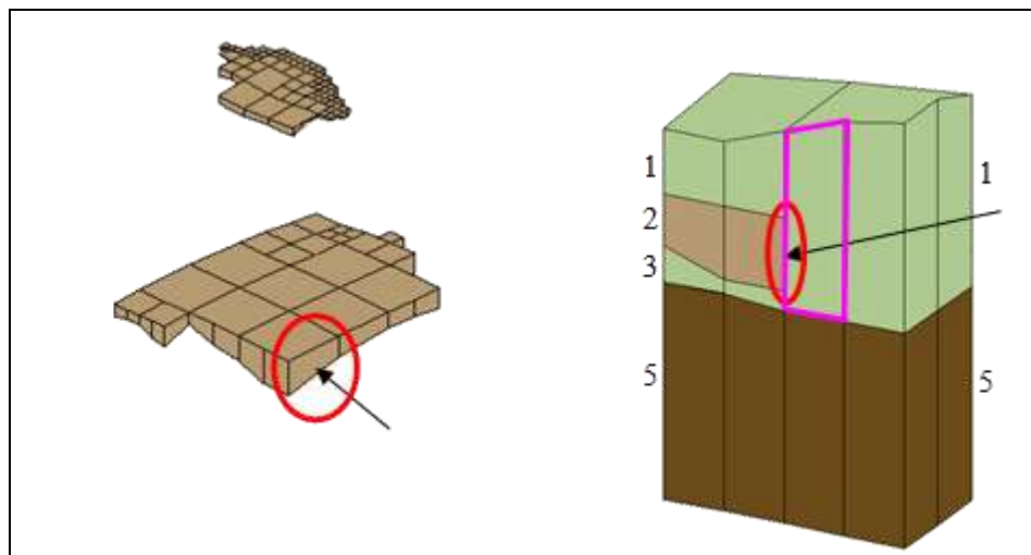
Figure 9 Layer 2 of 3D quadtree UGrid and side view cells
