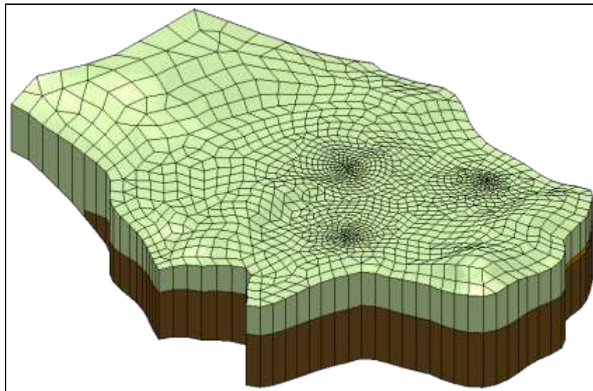
Figure 17 3D UGrid created from tri-quad 2D UGrid
