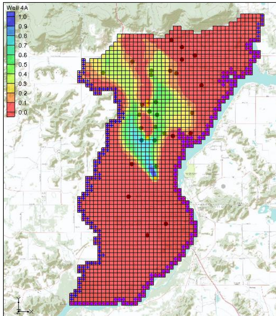
Figure 7 Probabilistic capture zone for proposed well
